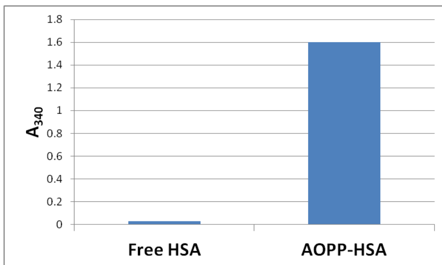
Figure 2. The AOPP-HSA Positive Control and untreated HSA were both prepared at a concentration of 100 \mu M and tested with STA-318 according to the assay protocol.
