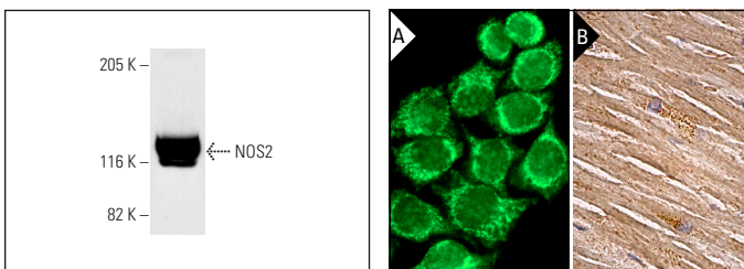
NOS2 (C-11): sc-7271. Western blot analysis of NOS2 expression in LPS and \gamma -interferon treated RAW 264.7 whole cell lysate.
