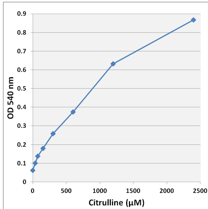
Figure 4. Citrulline standard curve.
