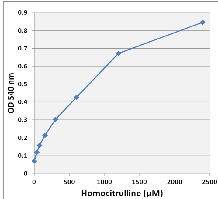
Figure 3. Homocitrulline standard curve.
