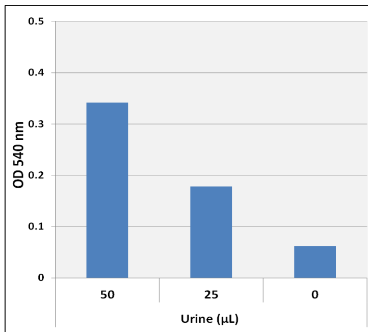
Figure 5. Detection of homocitrulline/citrulline in human urine.
