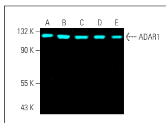
ADAR1 (15.8.6) Alexa Fluor® 647: sc-73408 AF647. Direct fluorescent western blot analysis of ADAR1 expression in NTERA-2 cl.D1 (A), Ramos (B), PC-3 (C), SK-BR-3 (D) and MOLT-4 (E) whole cell lysates. Blocked with UltraCruz® Blocking Reagent: sc-516214.
